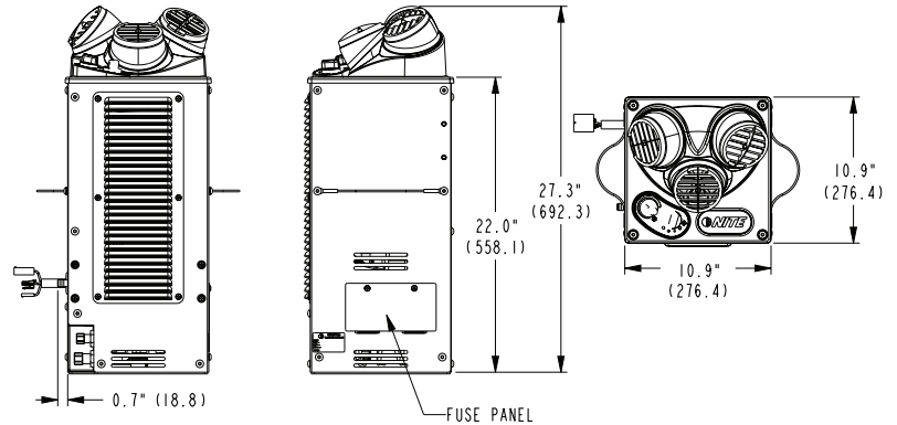
Interior Evaporator Unit
