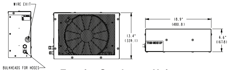
Exterior Condenser Unit
